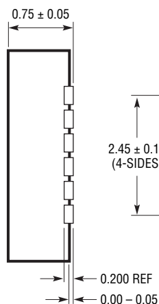
4.00 ± 0.10 (4 SIDES) PIN 1 TOP MARK (NOTE 6)
